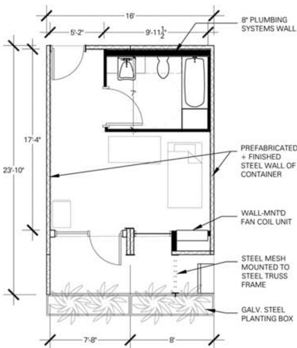
single bed handicap accessible suite prototype
