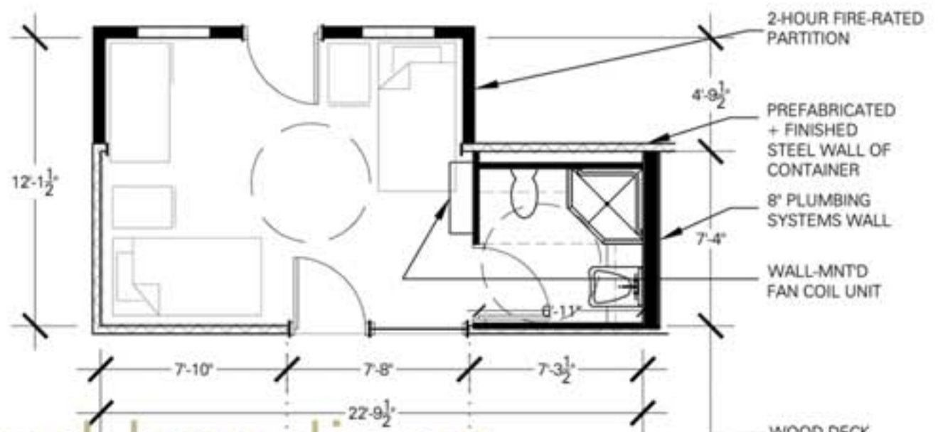
single bed suites prototype
