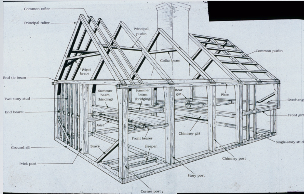
New England Box Frame and Earthfast Frame. Be prepared to name the framing members
