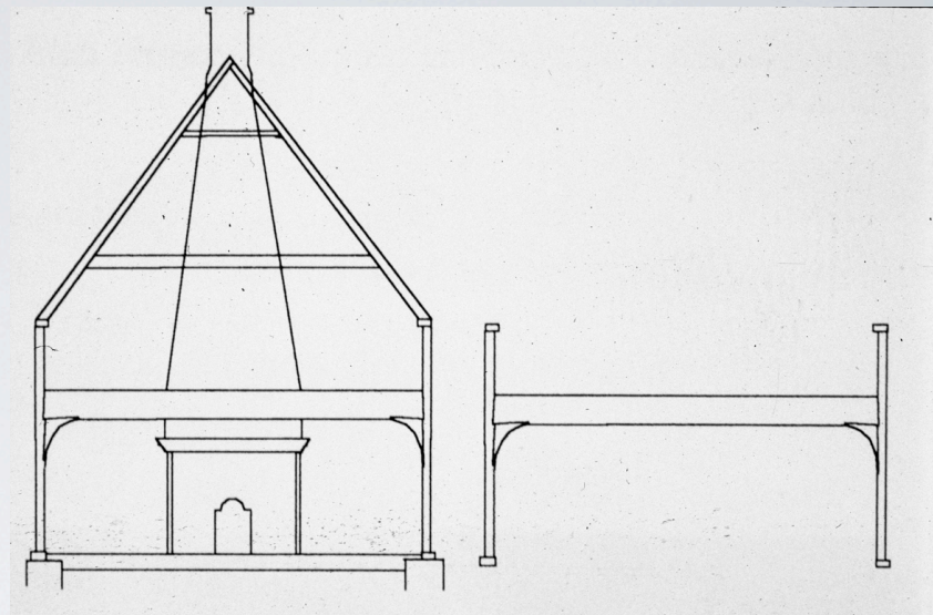
H-Bent or Anchor Balkan Frame of the Dutch House
